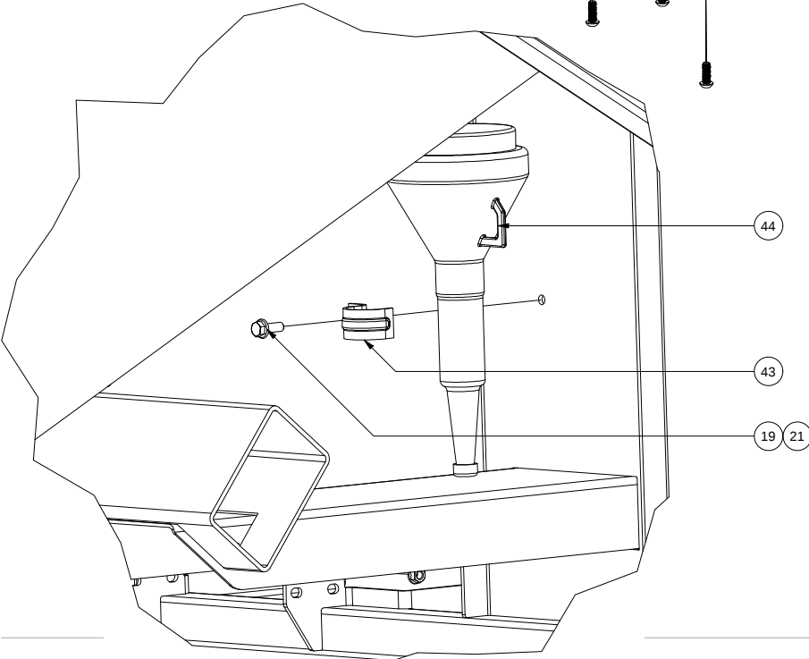
DETAIL B PAGE 8-9 FUEL FUNNEL PARTS HIDDEN FOR CLARITY
